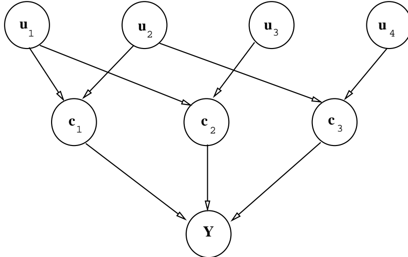
Figure 2: The Belief Network generated from the 2MONCNF formula \Sigma
